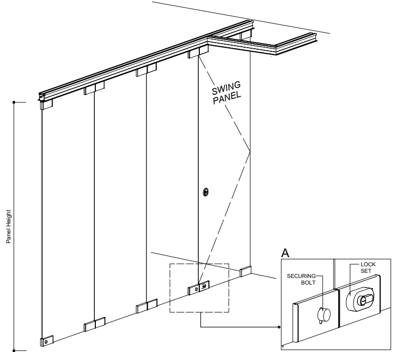
PERSPECTIVE ORDINARY CROSS TYPE SYSTEM
