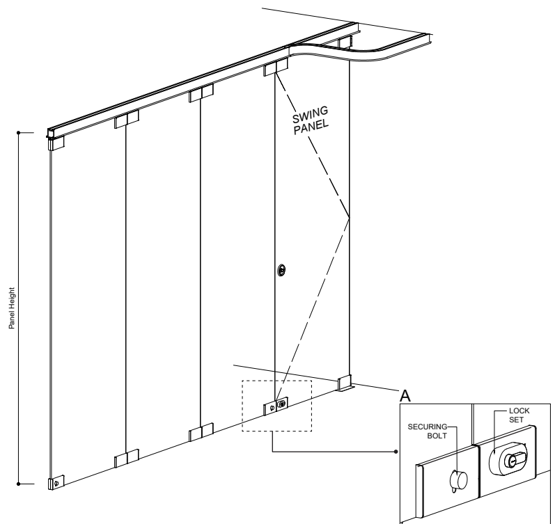
PERSPECTIVE ORDINARY STACKING R-TYPE SYSTEM
