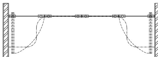
Double Stacking R-Type system
