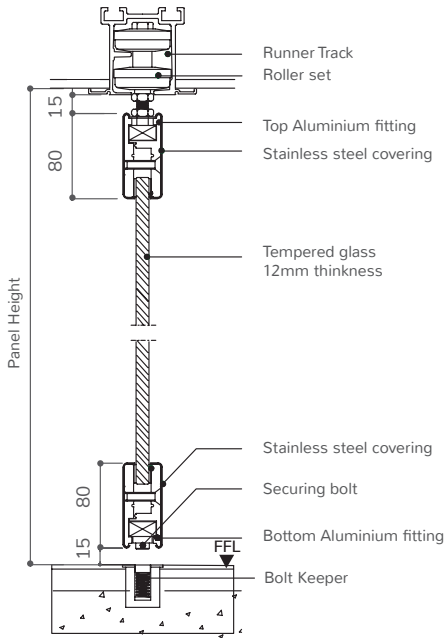
VERTICAL SECTION HORIZONTAL FRAME
