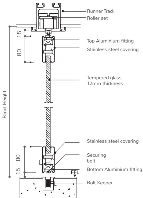
VERTICAL SECTION HORIZONTAL FRAME
